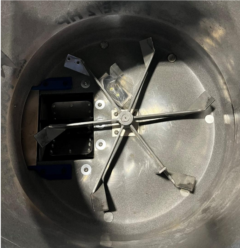
View of agitator & hopper ✓ New Agitator
